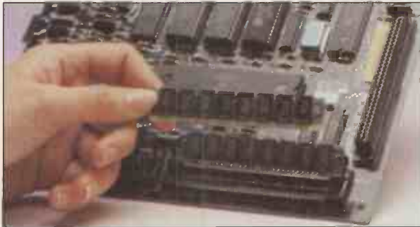
Above: A lot is packed into the limited space inside the SE. Right: The 256Kbit RAMs can be replaced by larger chips to boost the memory.
